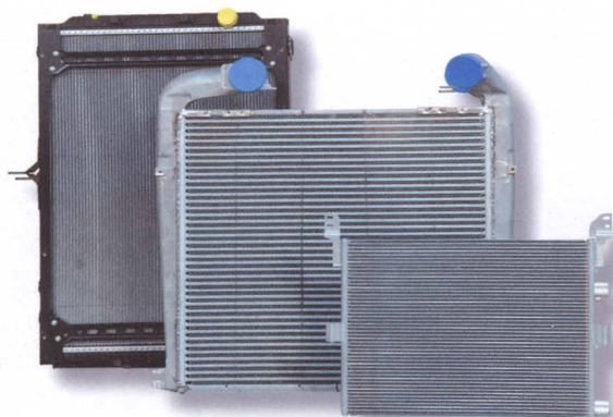
Radiateurs poids-lourds eau/air/clim Truck radiators water/intercooler/AC
